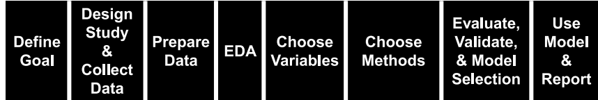
FIG. 2. Steps in the statistical modeling process.
